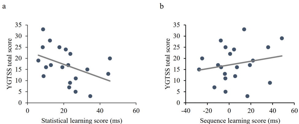
Figure 4. Correlation between (a) YGTSS total score and statistical learning score and (b) between YGTSS total score and sequence learning score. YGTSS = Yale Global Tic Severity Scale. Statistical learning score is the difference in RT between random high and random low-frequency triplets. Sequence learning score is the difference in RT between pattern high and random high-frequency triplets.
